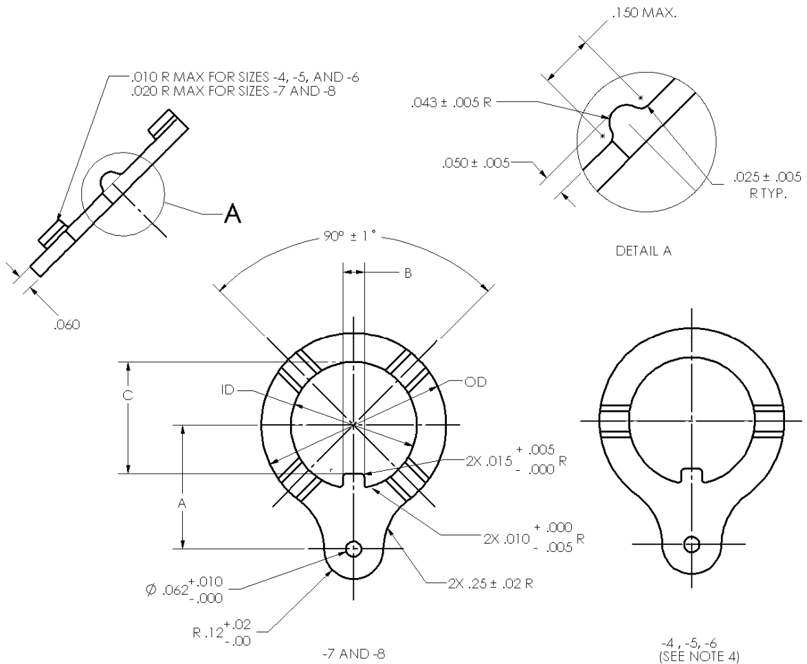
FIGURE 1 - LOCKING DEVICE
