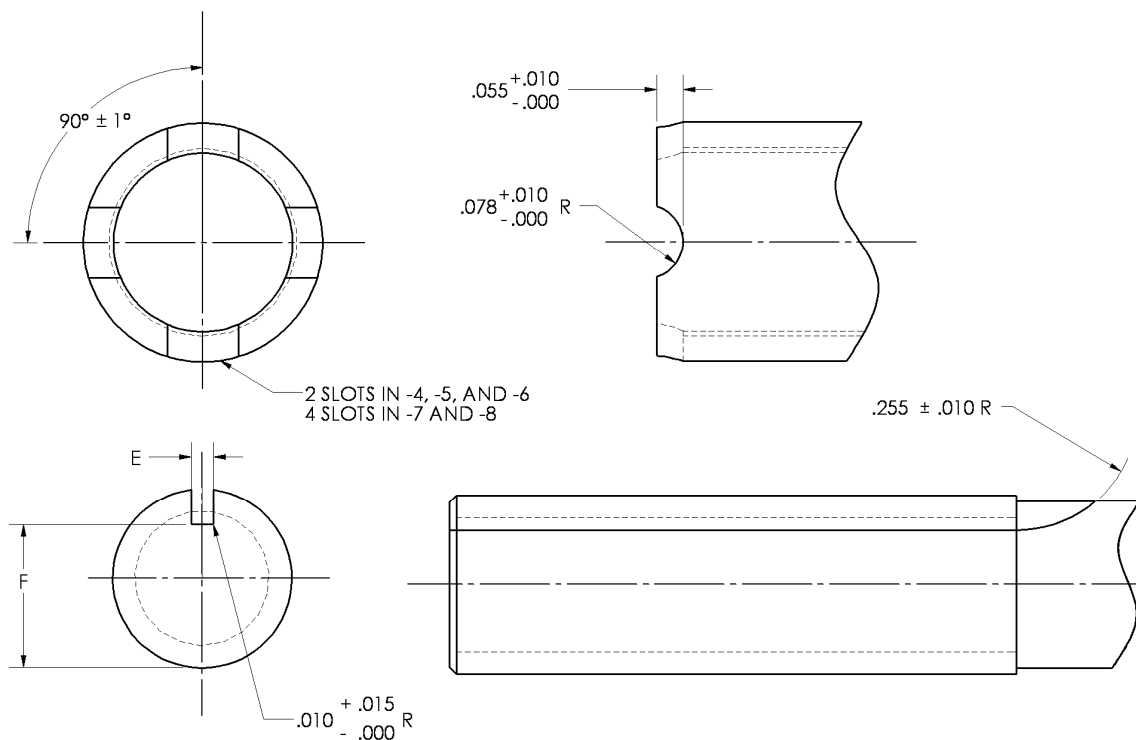
FIGURE 2 - ROD END TERMINAL DESIGN FOR USE WITH M81935/3 LOCKING DEVICE
