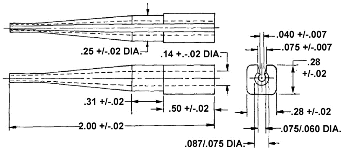
REMOVAL TOOL (-02)
