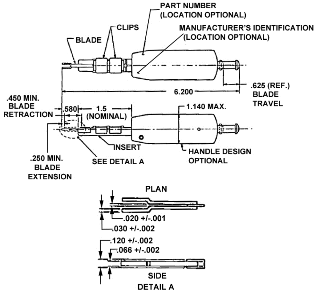
FIGURE 1 - REMOVAL TOOL CONFIGURATIONS/DIMENSIONS
