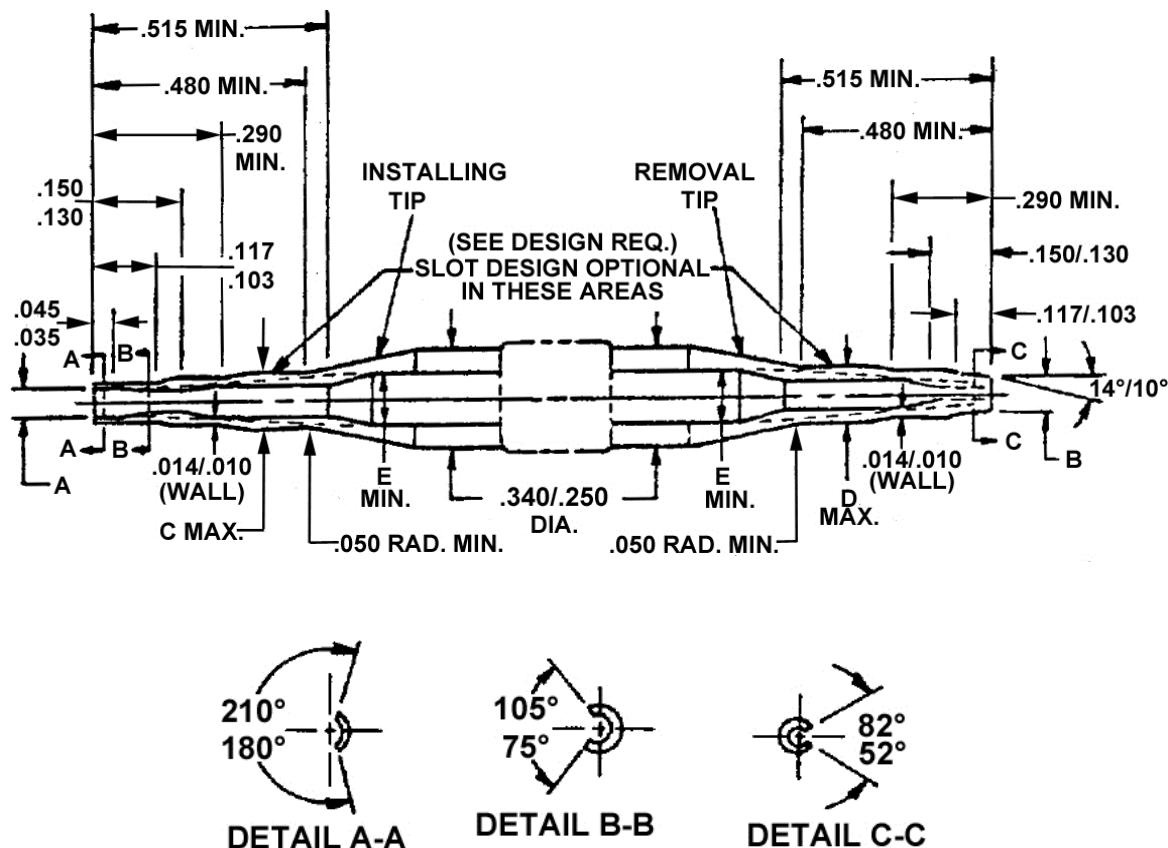
FIGURE 1 - INSTALLING AND REMOVAL TOOL (-01 AND -02)
