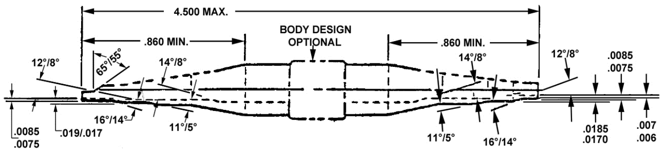
FIGURE 1 - INSTALLING AND REMOVAL TOOL (-01 AND -02) CONTINUED
