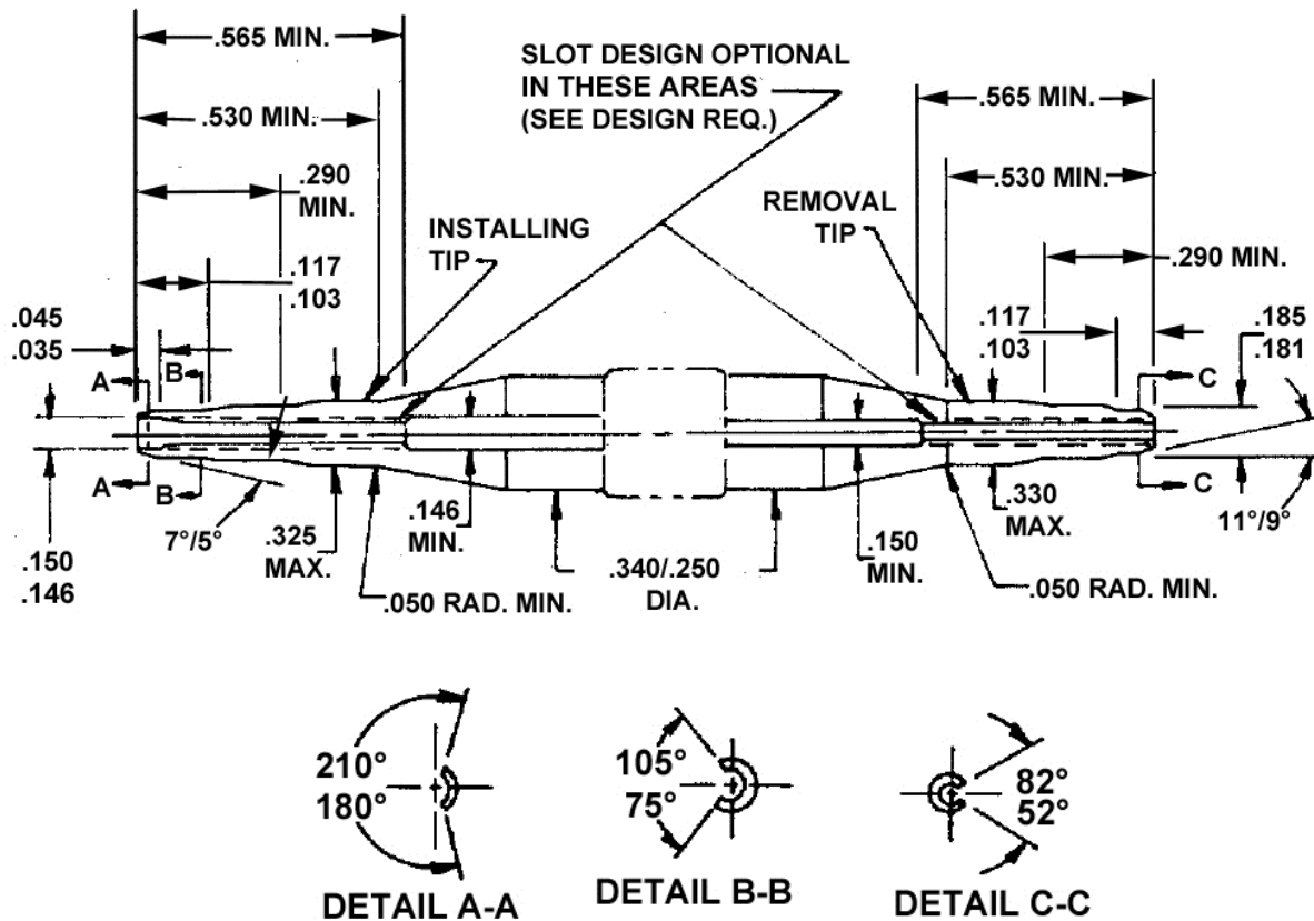
FIGURE 2 - INSTALLING AND REMOVAL TOOL (-03)
