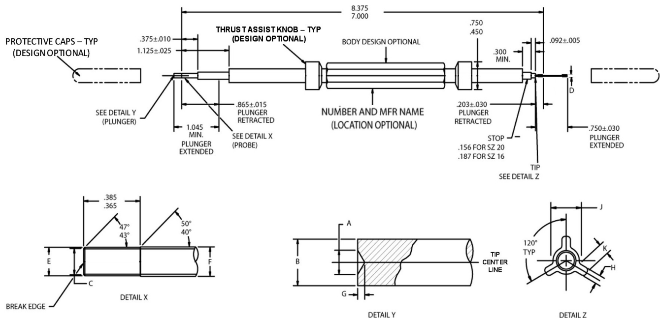
FIGURE 2 - REMOVAL TOOL -10 AND -11
