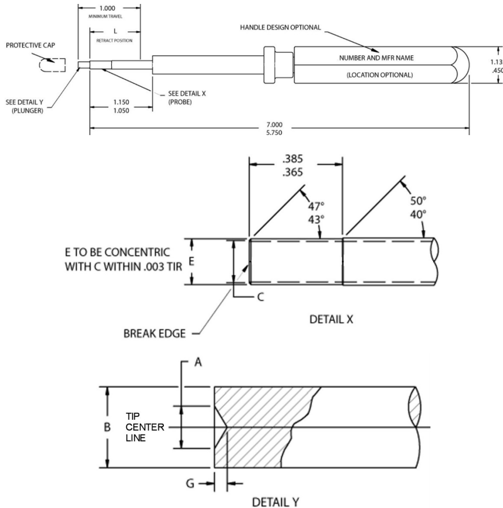
FIGURE 1 - REMOVAL TOOL -01 THRU -06
