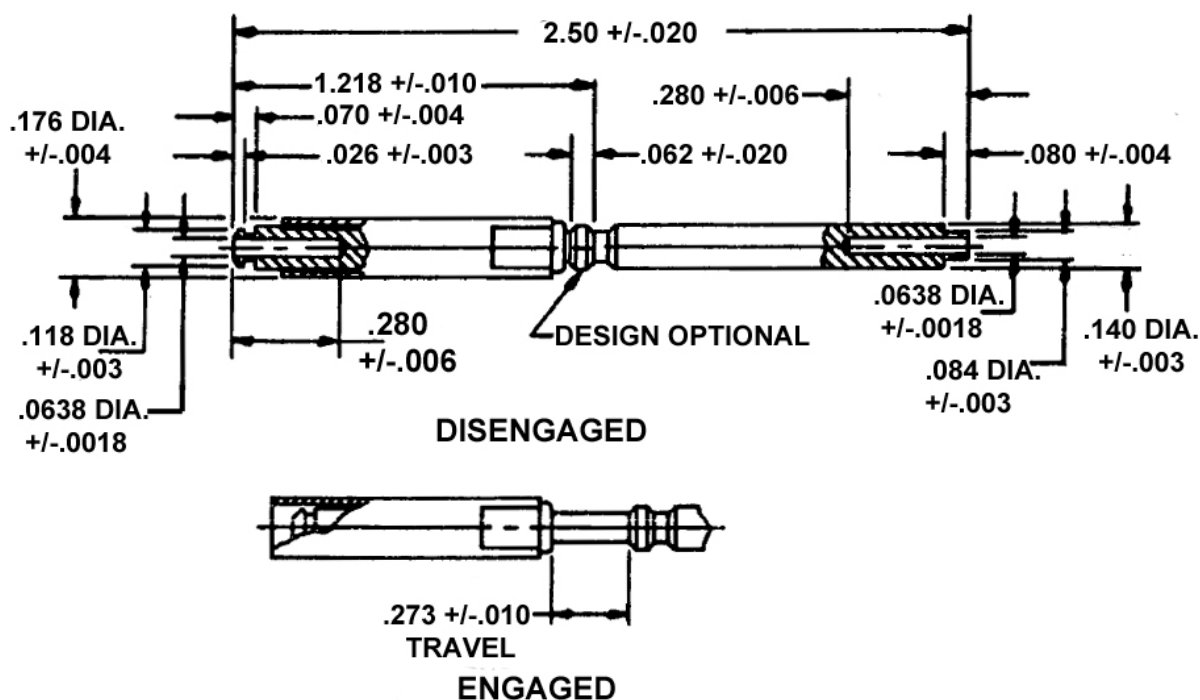
FIGURE 1 - INSTALLING AND REMOVAL TOOL CONFIGURATION AND DIMENSIONS
