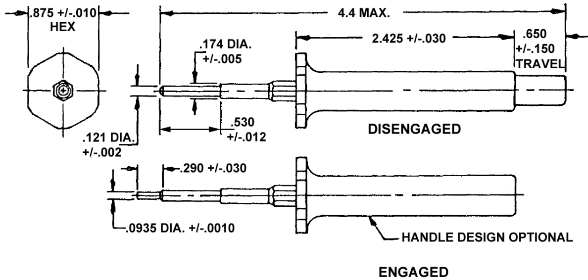
FIGURE 1 - REMOVAL TOOL CONFIGURATION AND DIMENSIONS
