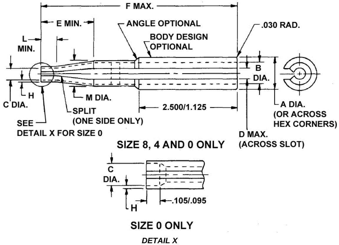
FIGURE 1 - REMOVAL TOOL CONFIGURATIONS/DIMENSIONS (DASH -02, -03, AND -04)
