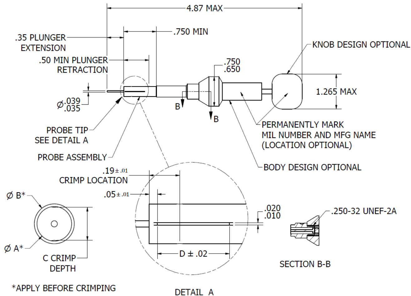
FIGURE 2 - TOOL CONFIGURATION (METAL TIP VERSION)
