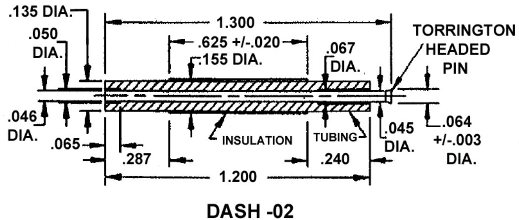
FIGURE 1 - REMOVAL TOOL -01 AND -02 CONFIGURATIONS AND DIMENSIONS
