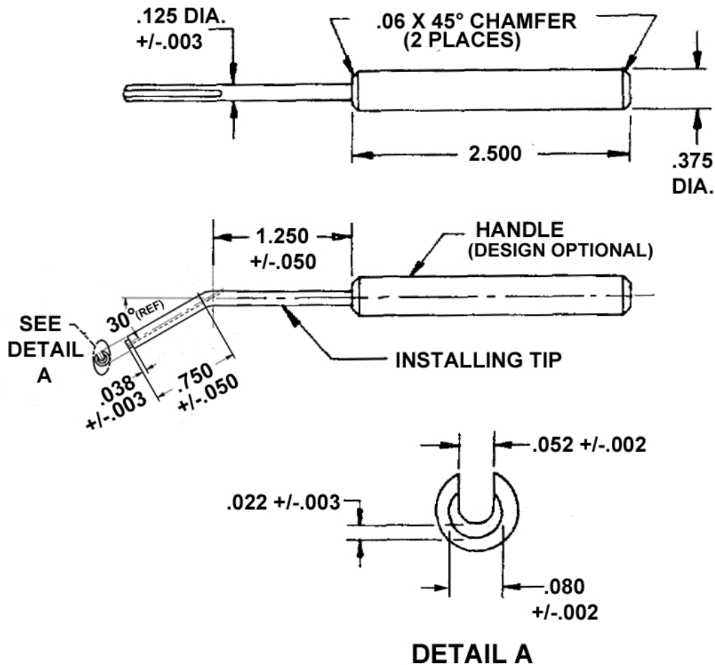
FIGURE 1 - INSTALLING TOOL CONFIGURATION AND DIMENSIONS
