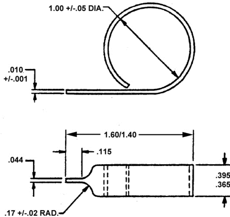
FIGURE 1 - TOOL CONFIGURATION AND DIMENSIONS
