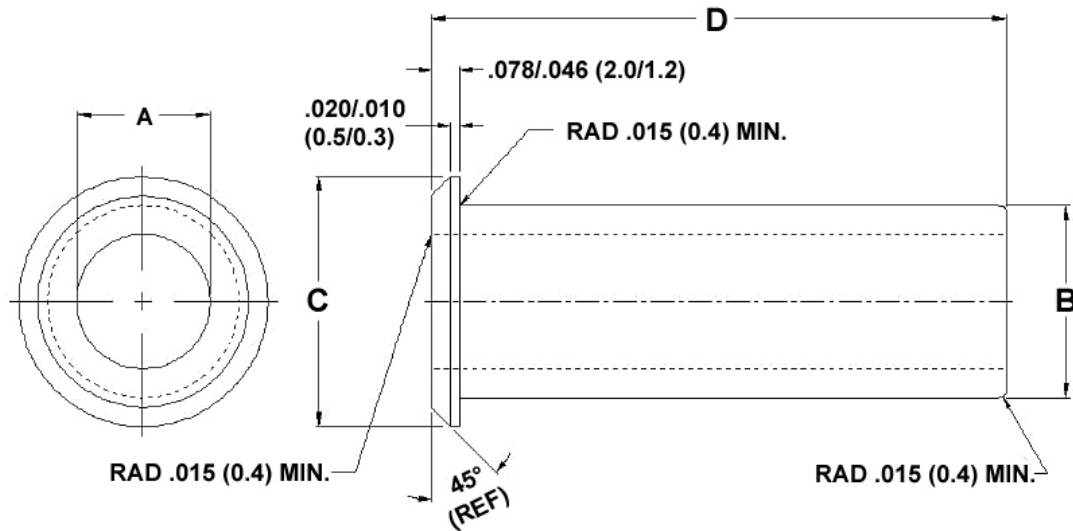
FIGURE 1 - BUSHING CONFIGURATION AND DIMENSIONS (WITH FLANGE)
