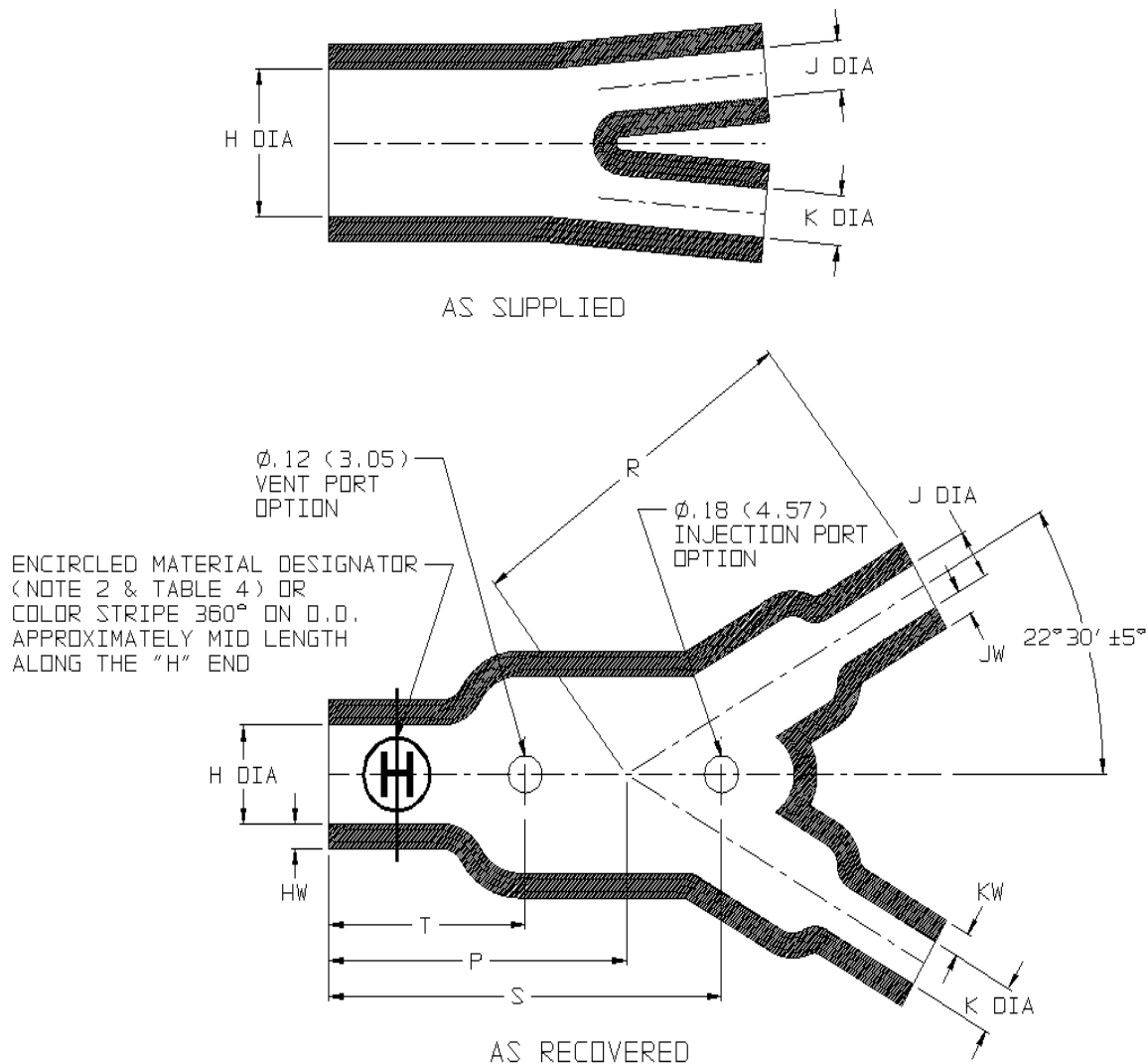
FIGURE 2 - BOOT, Y-TYPE (SEE TABLE 2)
