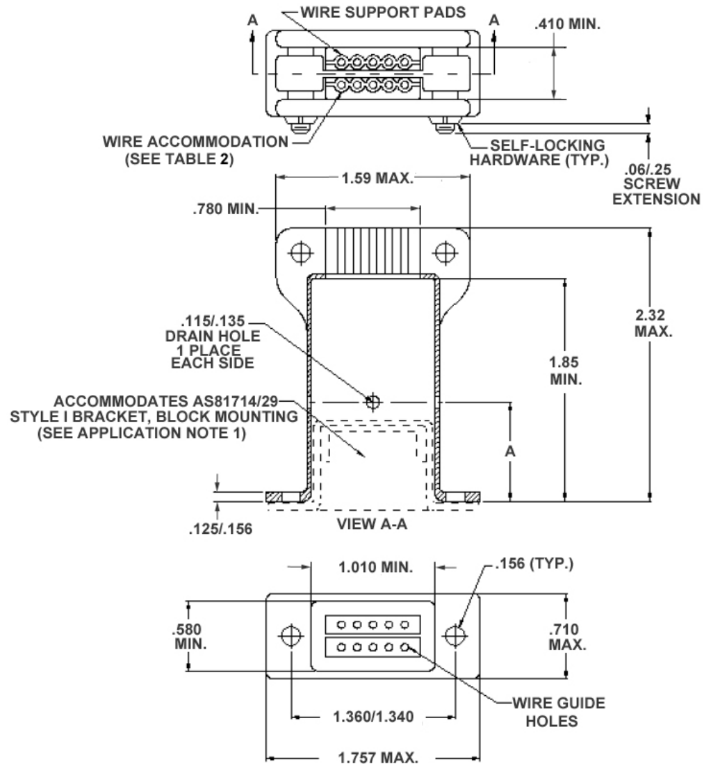
FIGURE 1 - BACKSHELL CONFIGURATION AND DIMENSIONS
