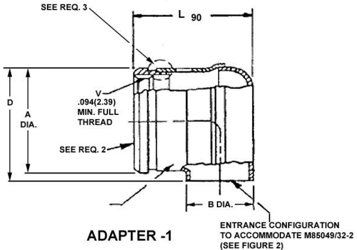
FIGURE 1 - ACCESSORY DIMENSIONS AND CONFIGURATION – 90 DEGREE ADAPTER
