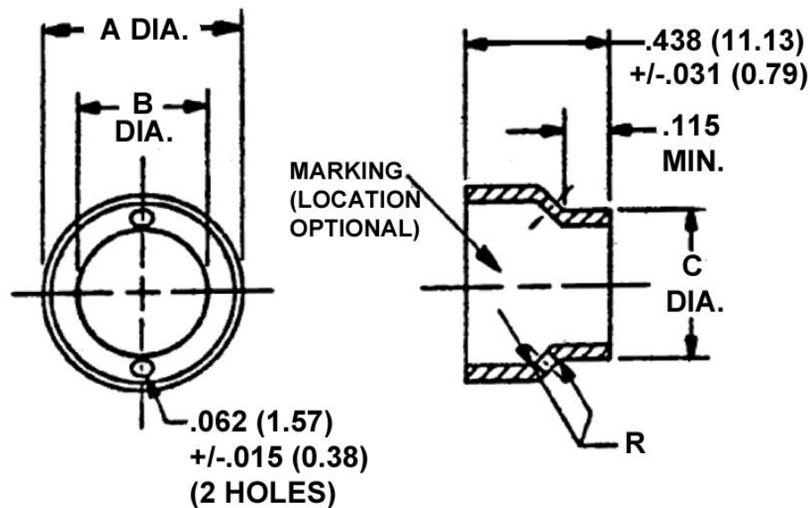
FIGURE 2 - DIMENSIONS AND CONFIGURATION - ADAPTER REDUCER
