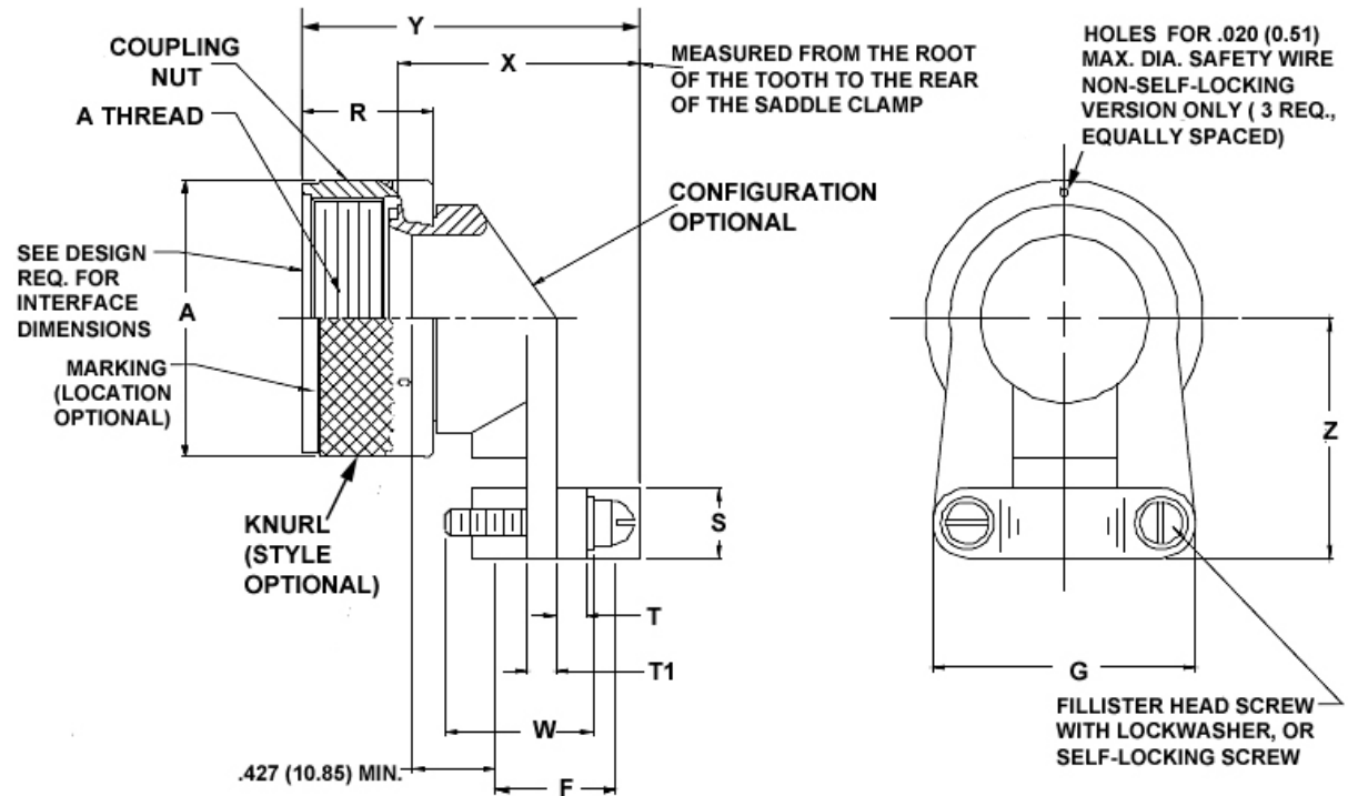
FIGURE 1 - ACCESSORY CONFIGURATION AND DIMENSIONS (NON-SELF-LOCKING AND SELF-LOCKING)
