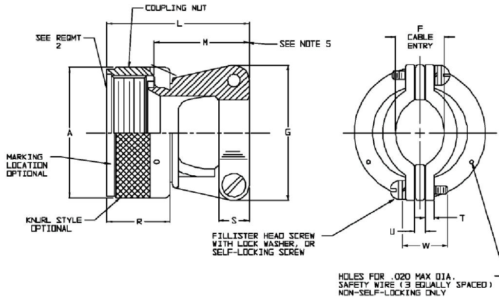
FIGURE 1 - ACCESSORY CONFIGURATION AND DIMENSIONS (NON-SELF-LOCKING OR SELF-LOCKING COUPLING)
