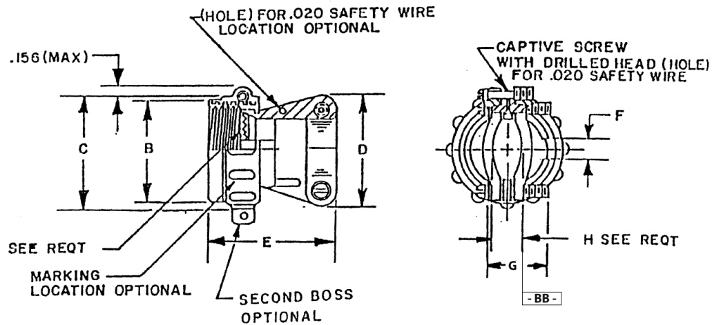
FIGURE 1 – DIMENSIONS AND CONFIGURATION
