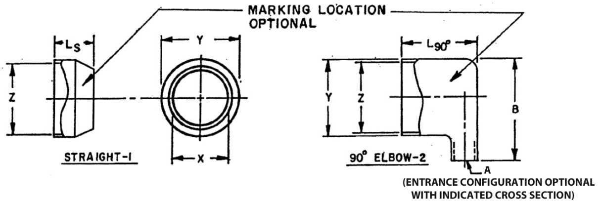
FIGURE 1 – DIMENSIONS AND CONFIGURATION
