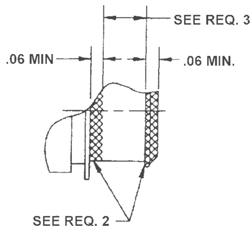
FIGURE 2 - SELECTIVE PLATING
