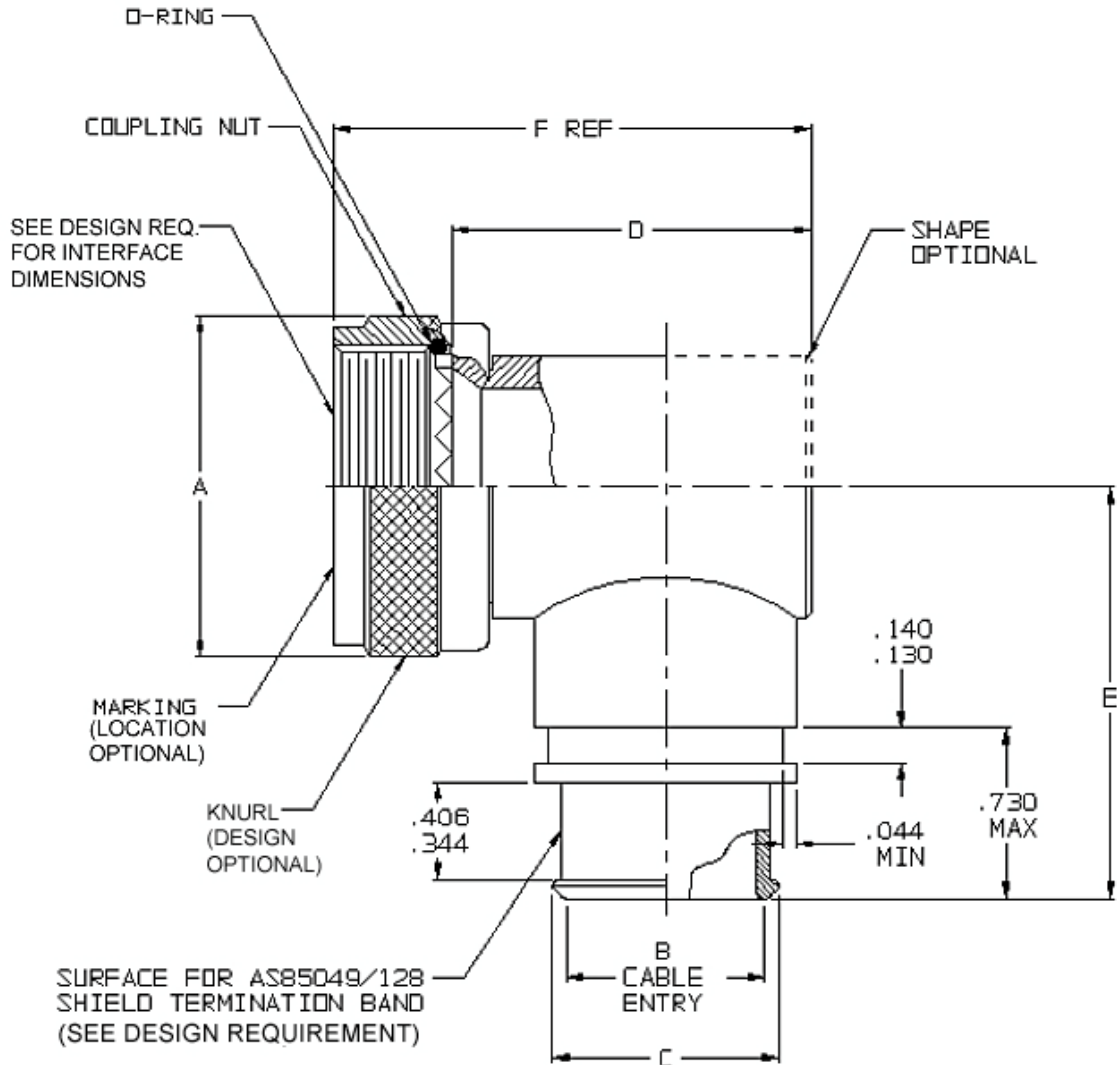
FIGURE 1 - ACCESSORY CONFIGURATION AND DIMENSIONS
