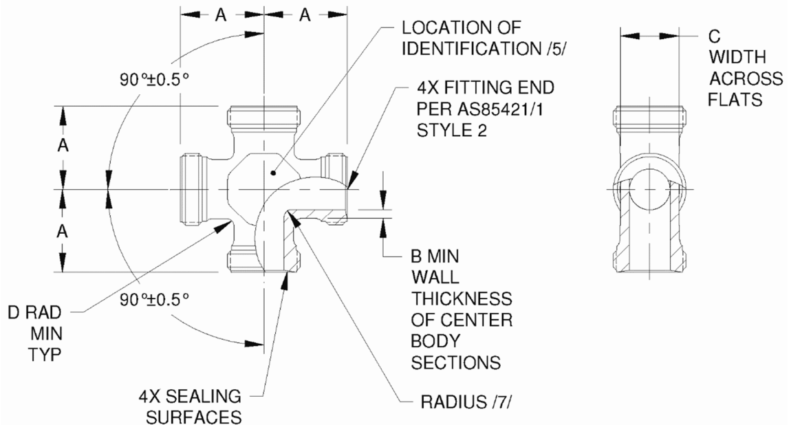
FIGURE 1 - FITTING, CROSS
