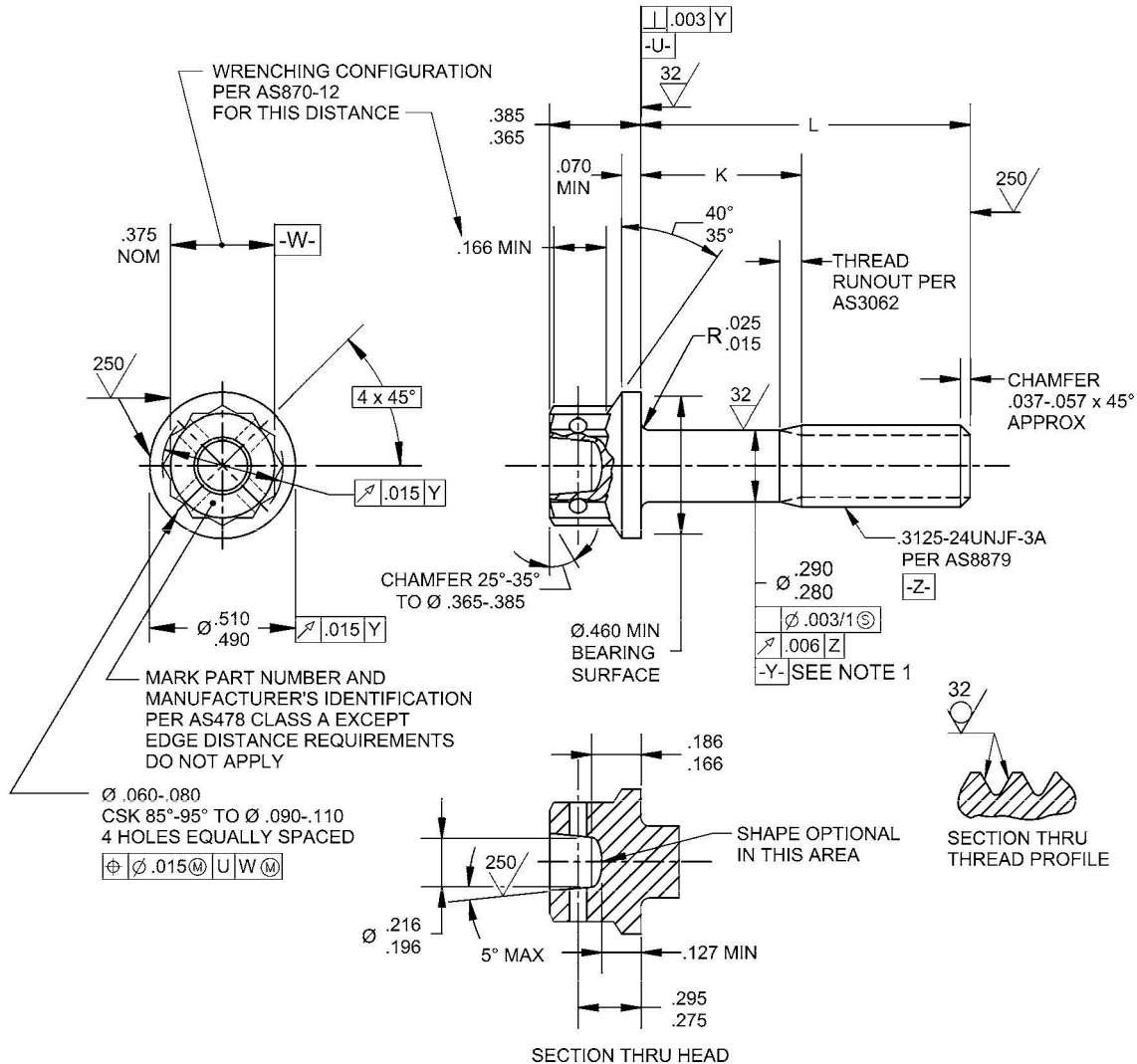
FIGURE 1 - BOLT
