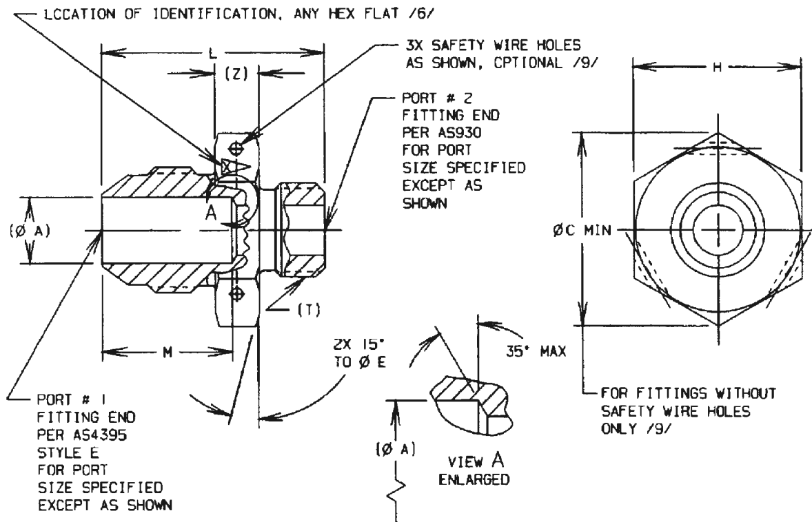
FIGURE 1 - FITTING, ADAPTER, REDUCER
