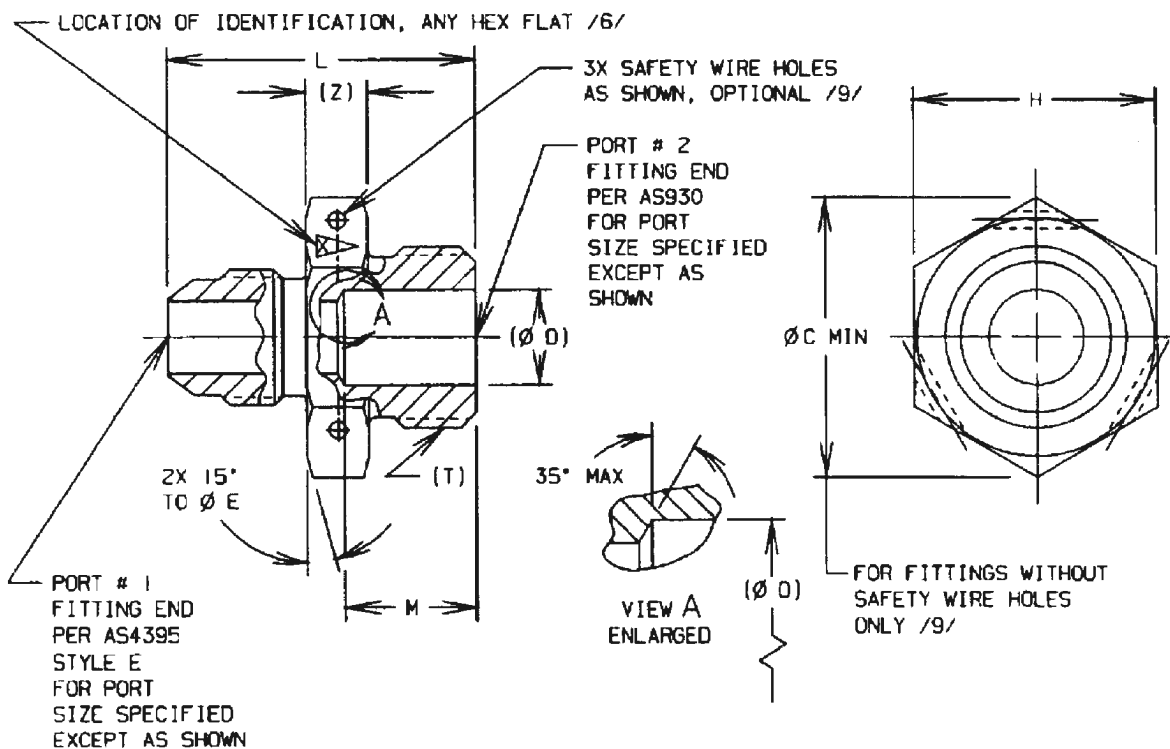
FIGURE 2 - FITTING, ADAPTER, EXPANDER
