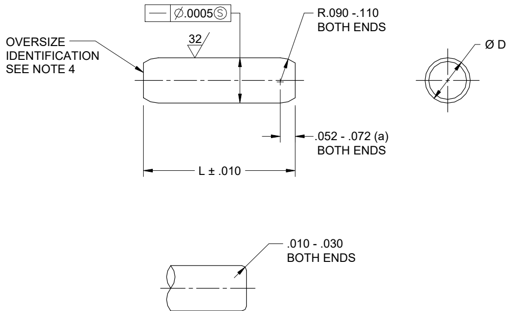
(a) VIEW SHOWING ROUNDING OF ENDS FOR PIN DIAMETERS LESS THAN .12500
