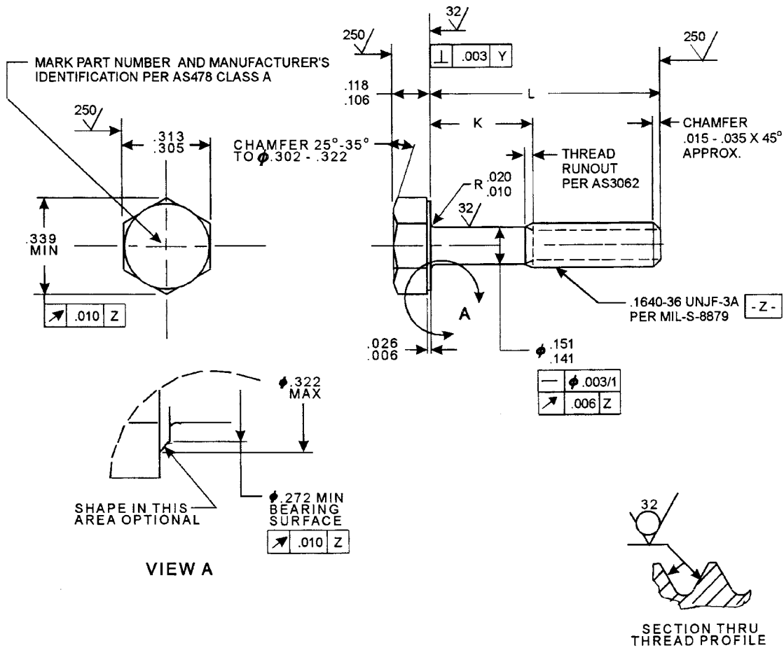
FIGURE 1 - SCREW
