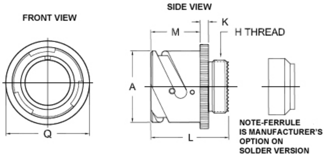
FIGURE 1 - CONNECTOR RECEPTACLE
