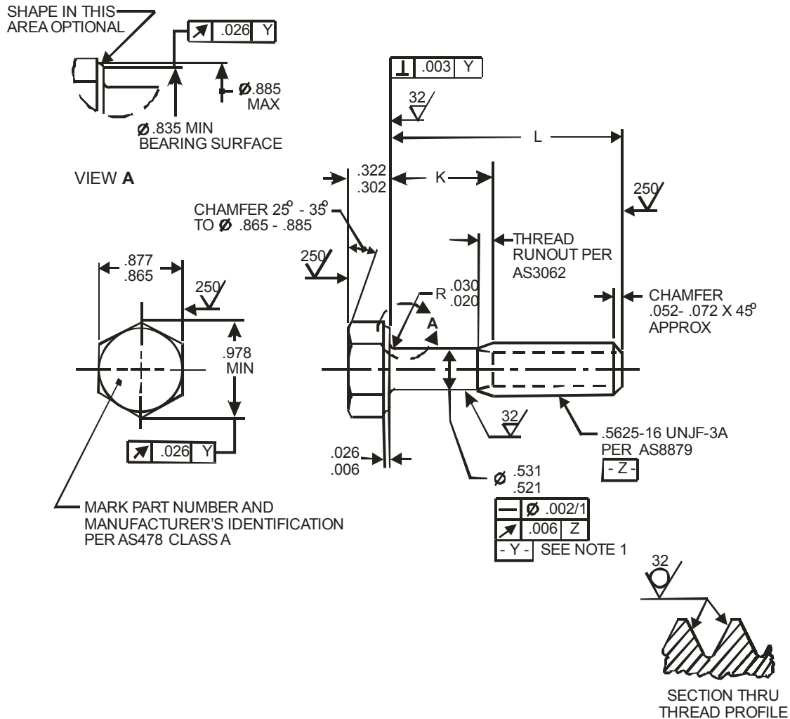
FIGURE 1 - BOLT
