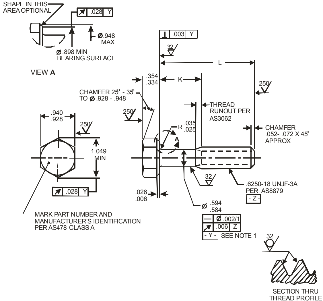
FIGURE 1 - BOLT
