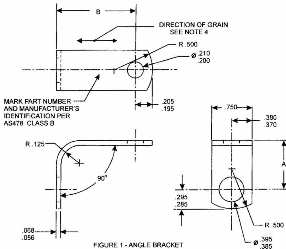
FIGURE 1 - ANGLE BRACKET
