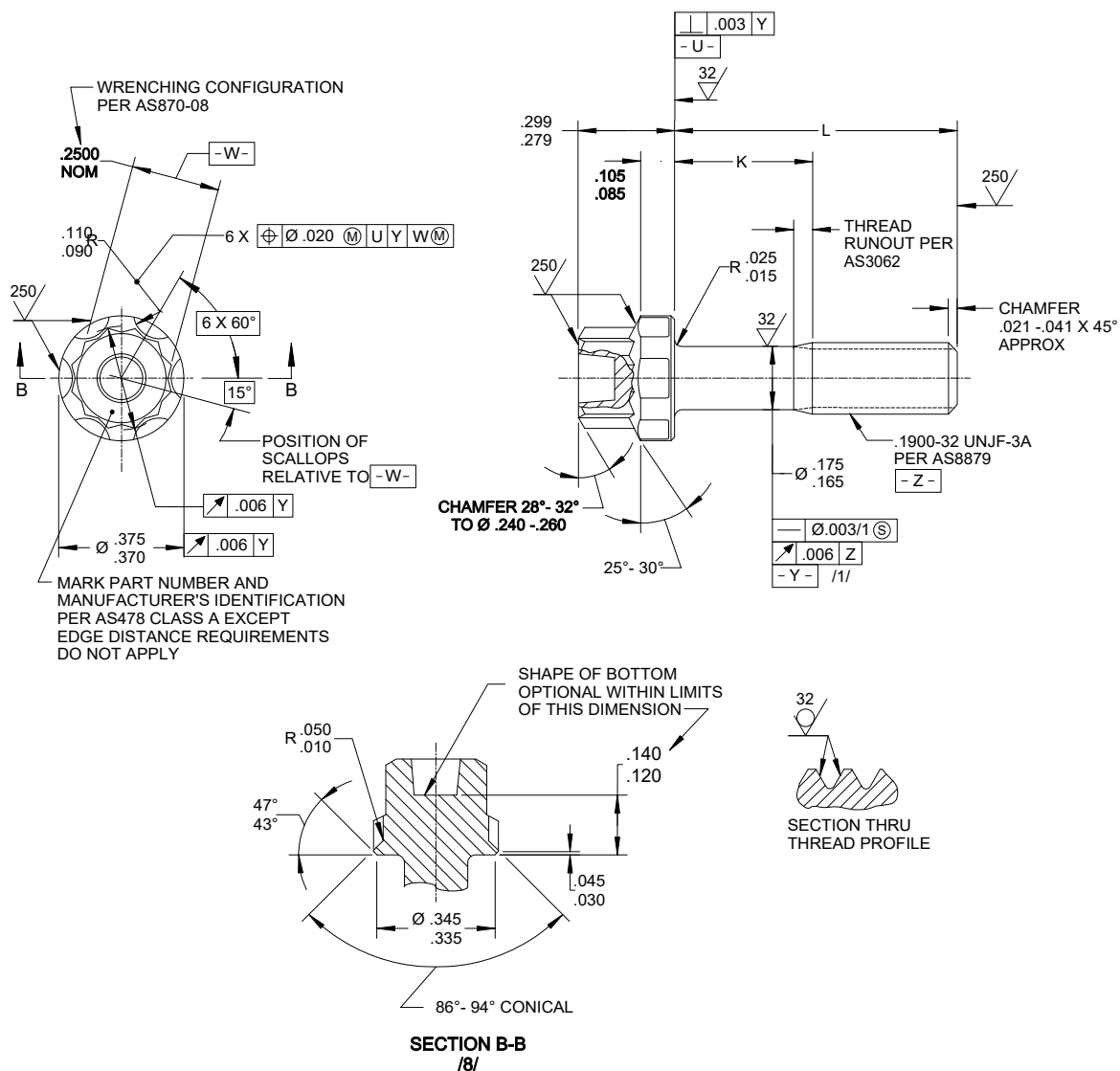
FIGURE 1 - BOLT
