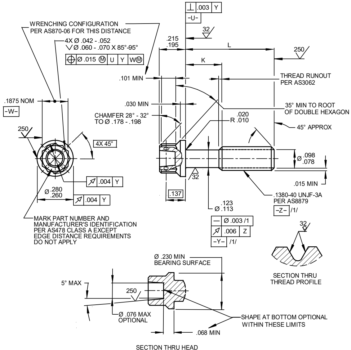
FIGURE 1 - BOLT
