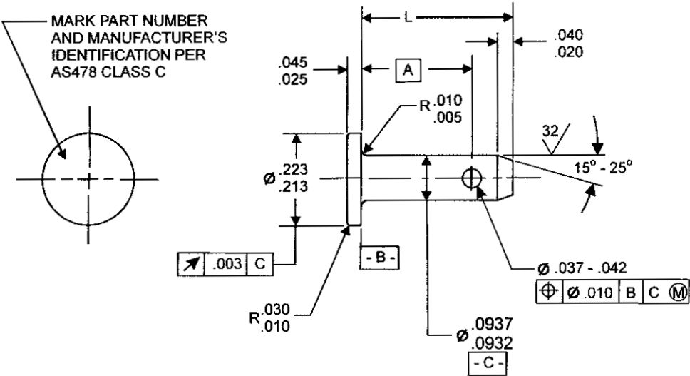
FIGURE 1 - PIN TABLE 1 - PART NUMBERS AND DIMENSIONS.
