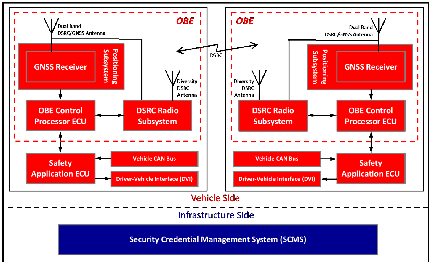
Figure 1 - On-board V2V system
