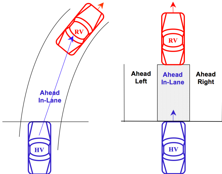
Figure 8 - Relevant RV zones for FCW feature
