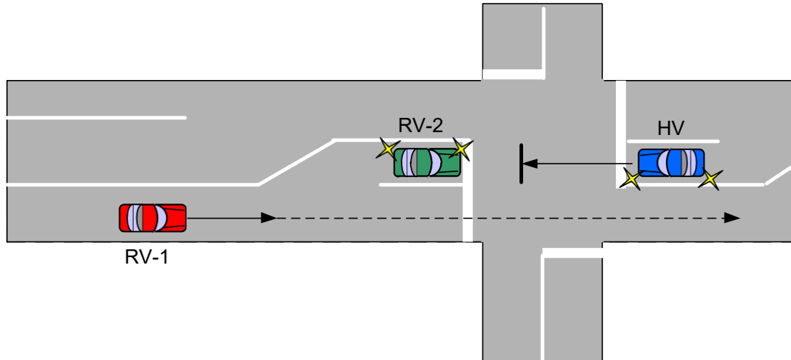
Figure 15 - LTA - left turn across path
