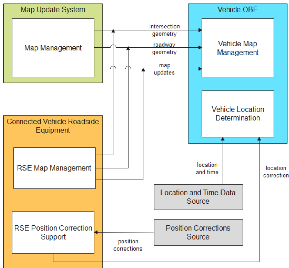
Figure 2 - ARC-IT objects and data flows
