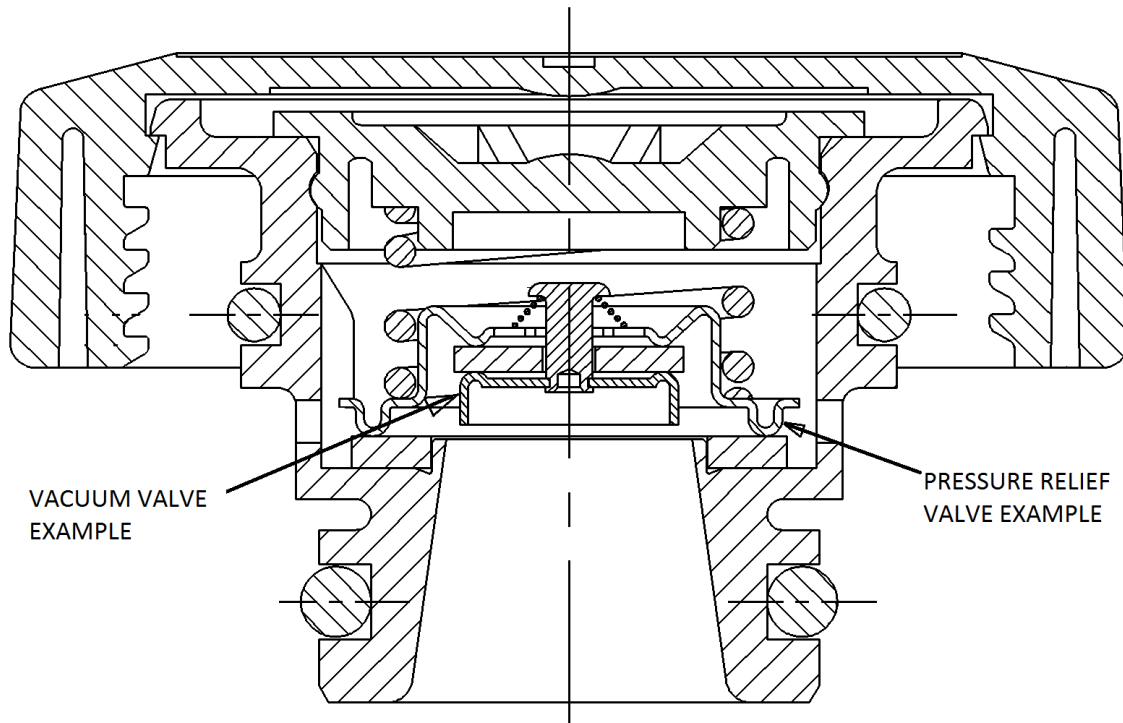
Figure 1 - Section view of typical pressure cap
