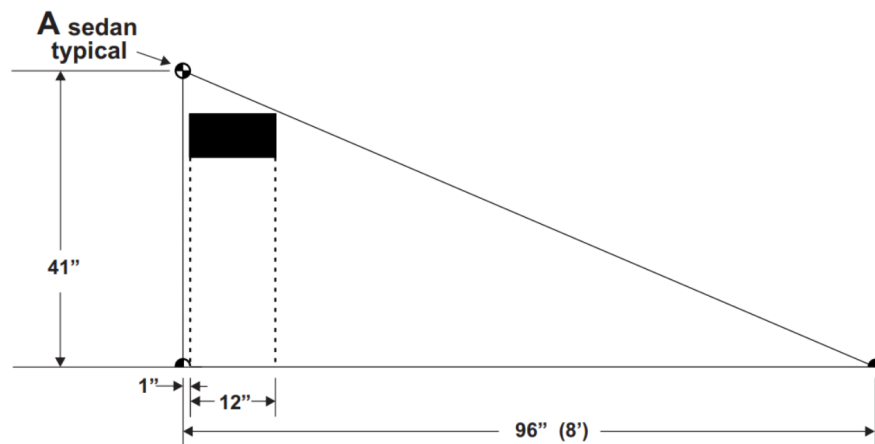
Figure 10 - Image size test object with the field of view target for a typical sedan
