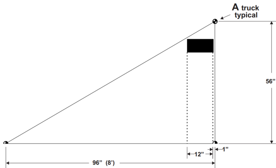
Figure 14 - Image size test object with the field of view target for a typical pickup truck
