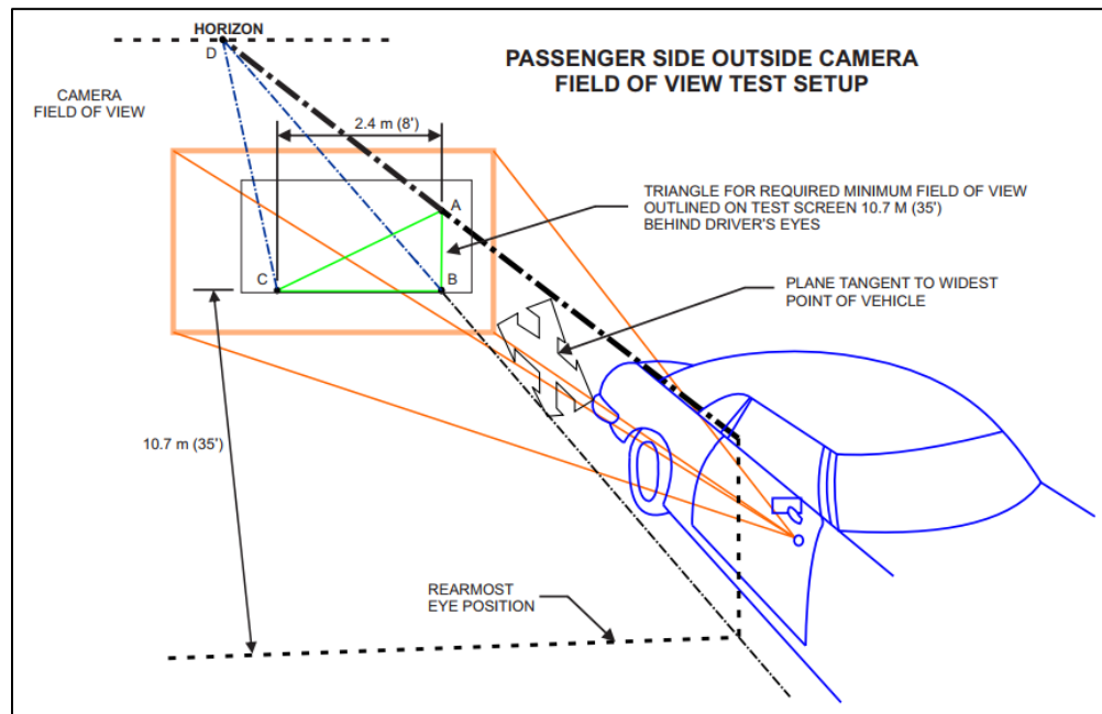
Figure 4 - Verification test - Method A, physical test
