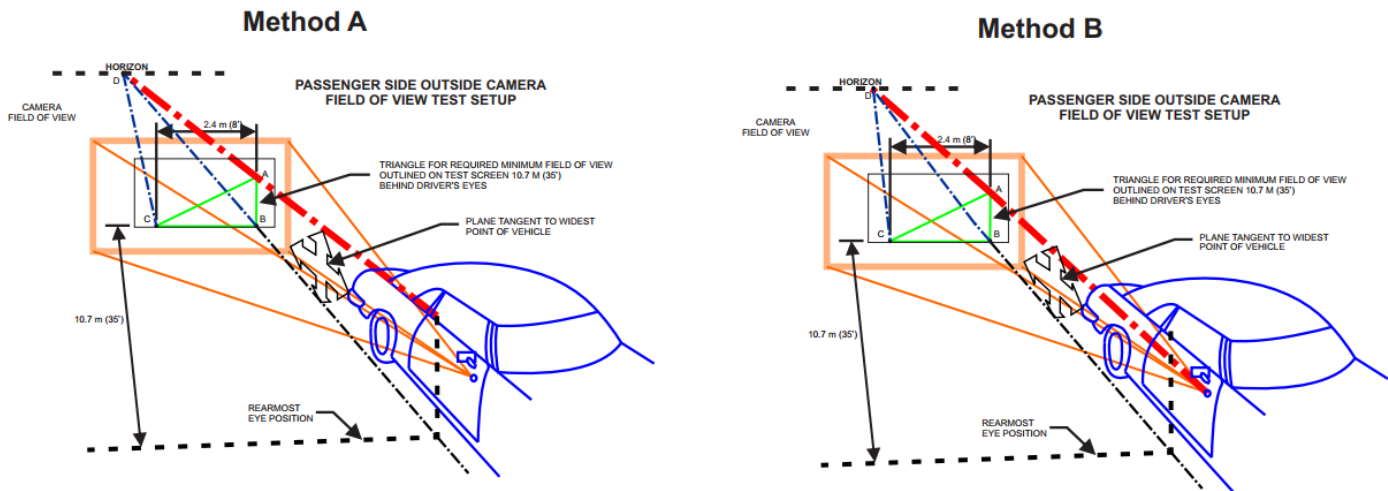
Figure 6 - Comparison of Method A and Method B physical tests
