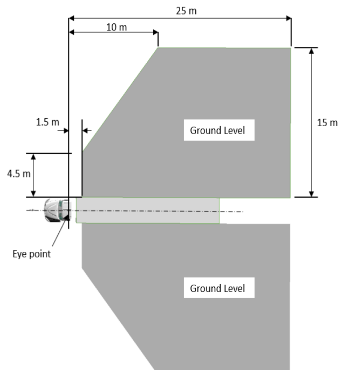
Figure 9 - Heavy truck field of view - wide-angle view
