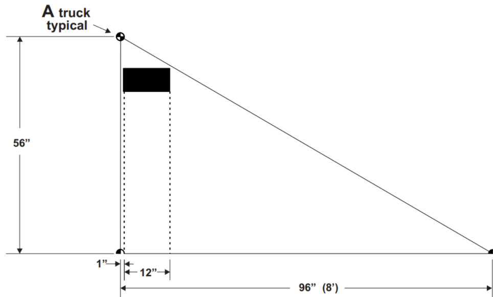
Figure 11 - Image size test object with the field of view target for a typical pickup truck
