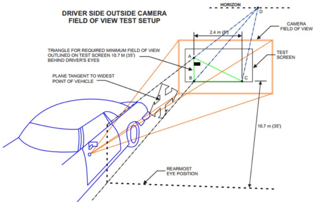
Figure 12 - Image size test object with the field of view target - driver's side
