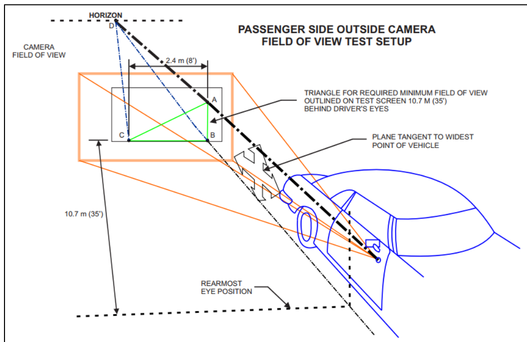
Figure 5 - Verification test - Method B, physical test
