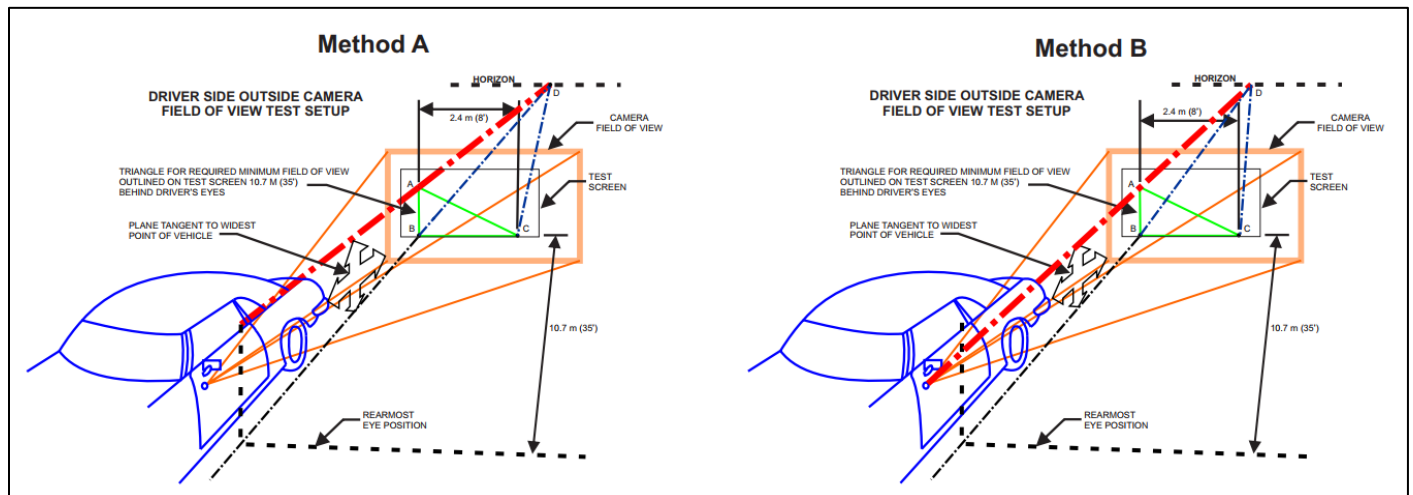
Figure 3 - Comparison of Method A and Method B physical tests
