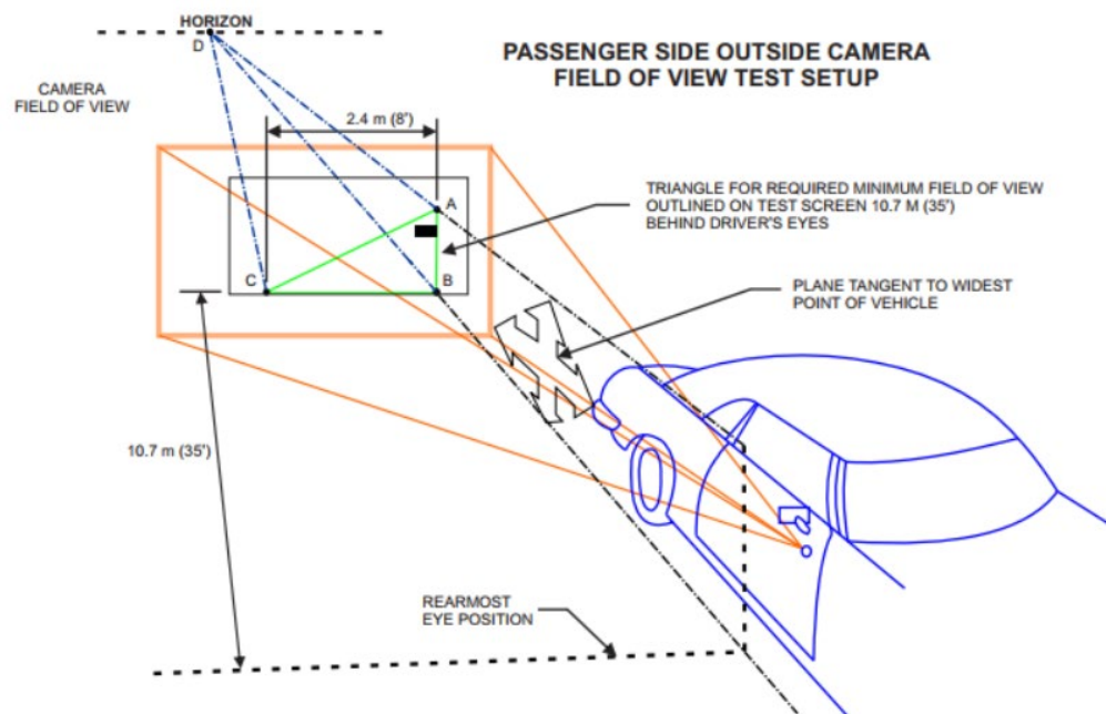
Figure 15 - Image size test object with the field of view target - passenger's side
