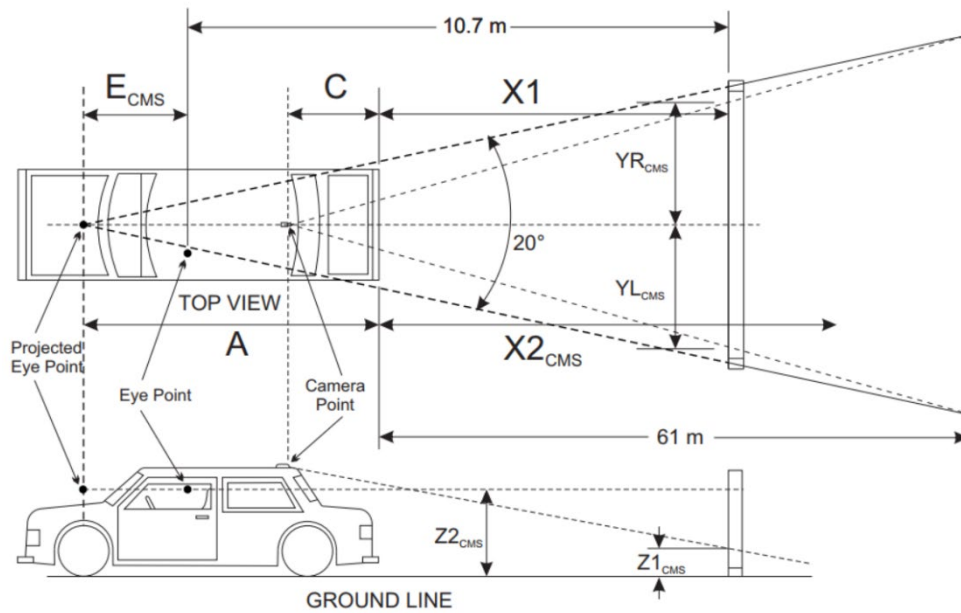
Figure 7 - Verification test - physical test
