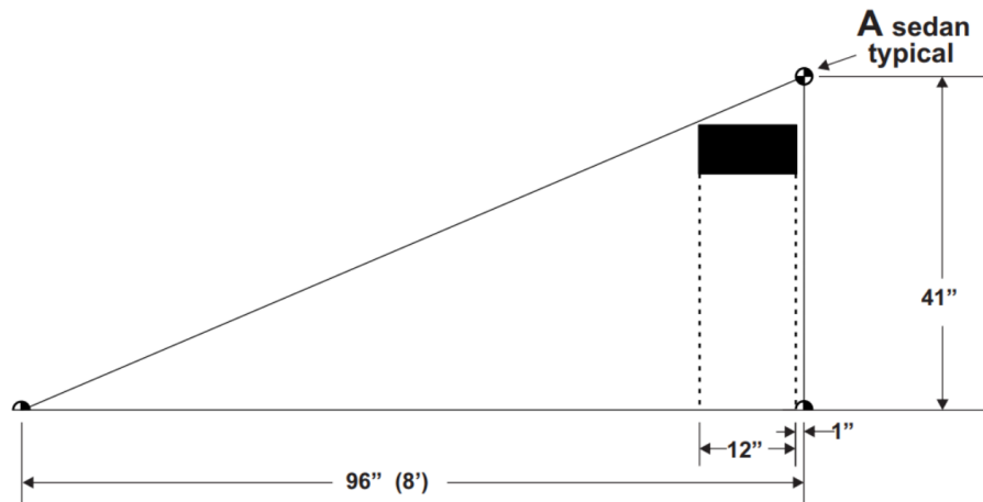
Figure 13 - Image size test object with the field of view target for a typical sedan
