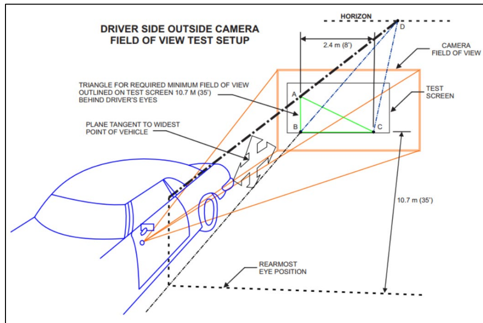
Figure 1 - Verification test - Method A, physical test
