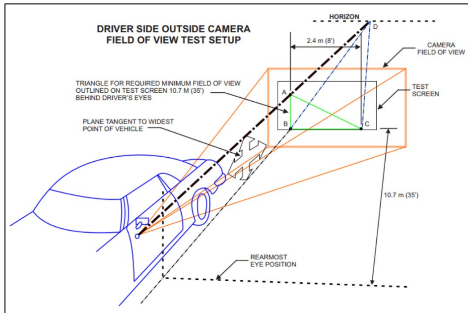
Figure 2 - Verification test - Method B, physical test
