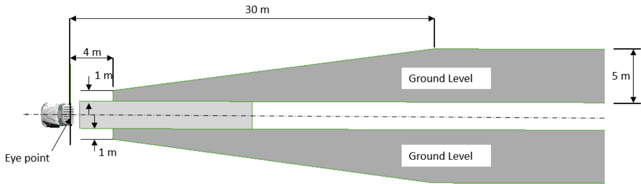
Figure 8 - Heavy truck field of view - main view
