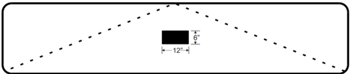
Figure 16 - Image size test object with the field of view target
