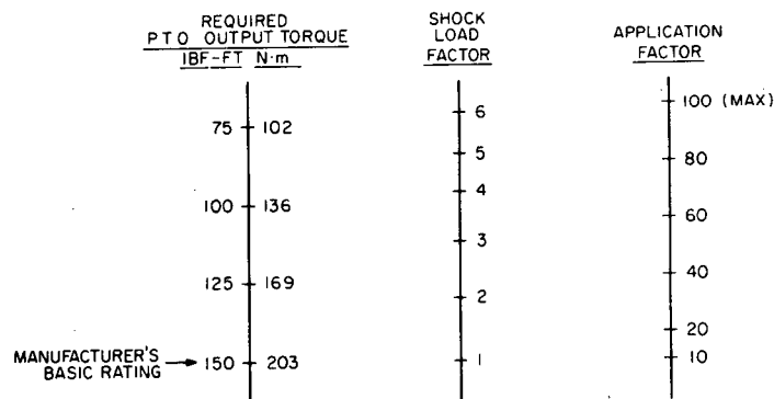
FIG. 1- EXAMPLE OF NOMOGRAM
