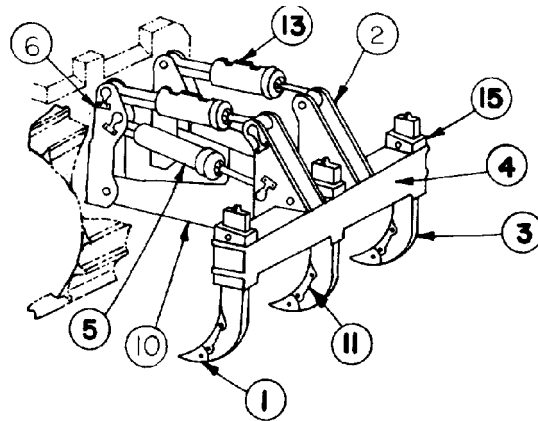
FIGURE 2—MULTI-SHANK VARIABLE PITCH PARALLELOGRAM RIPPER
