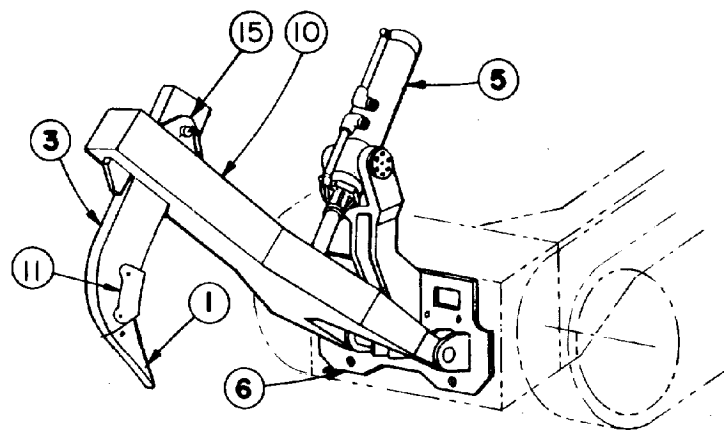
FIGURE 5—SINGLE SHANK RADIAL RIPPER
