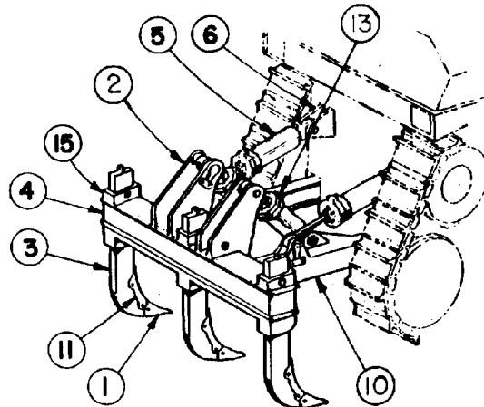
FIGURE 3—MULTI-SHANK VARIABLE PITCH RADIAL RIPPER
