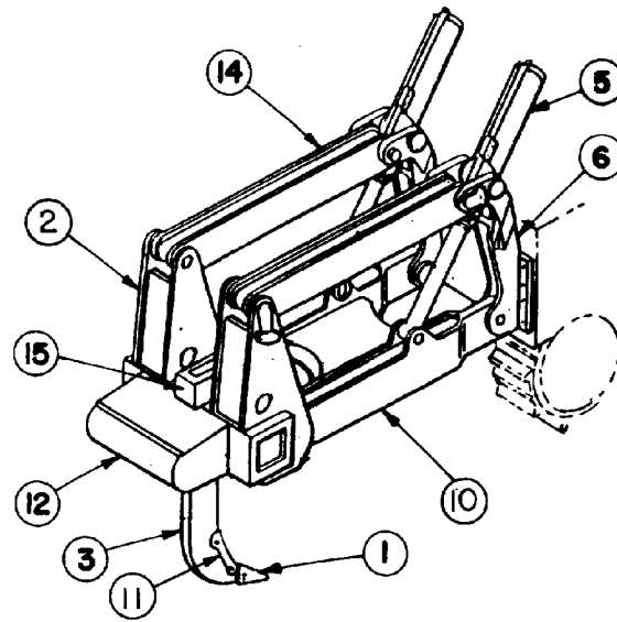
FIGURE 4—SINGLE SHANK PARALLELOGRAM RIPPER
