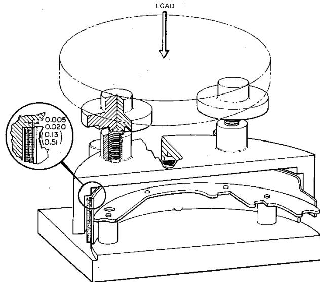
Figure 1 - Bond plane shear test - drum brake
