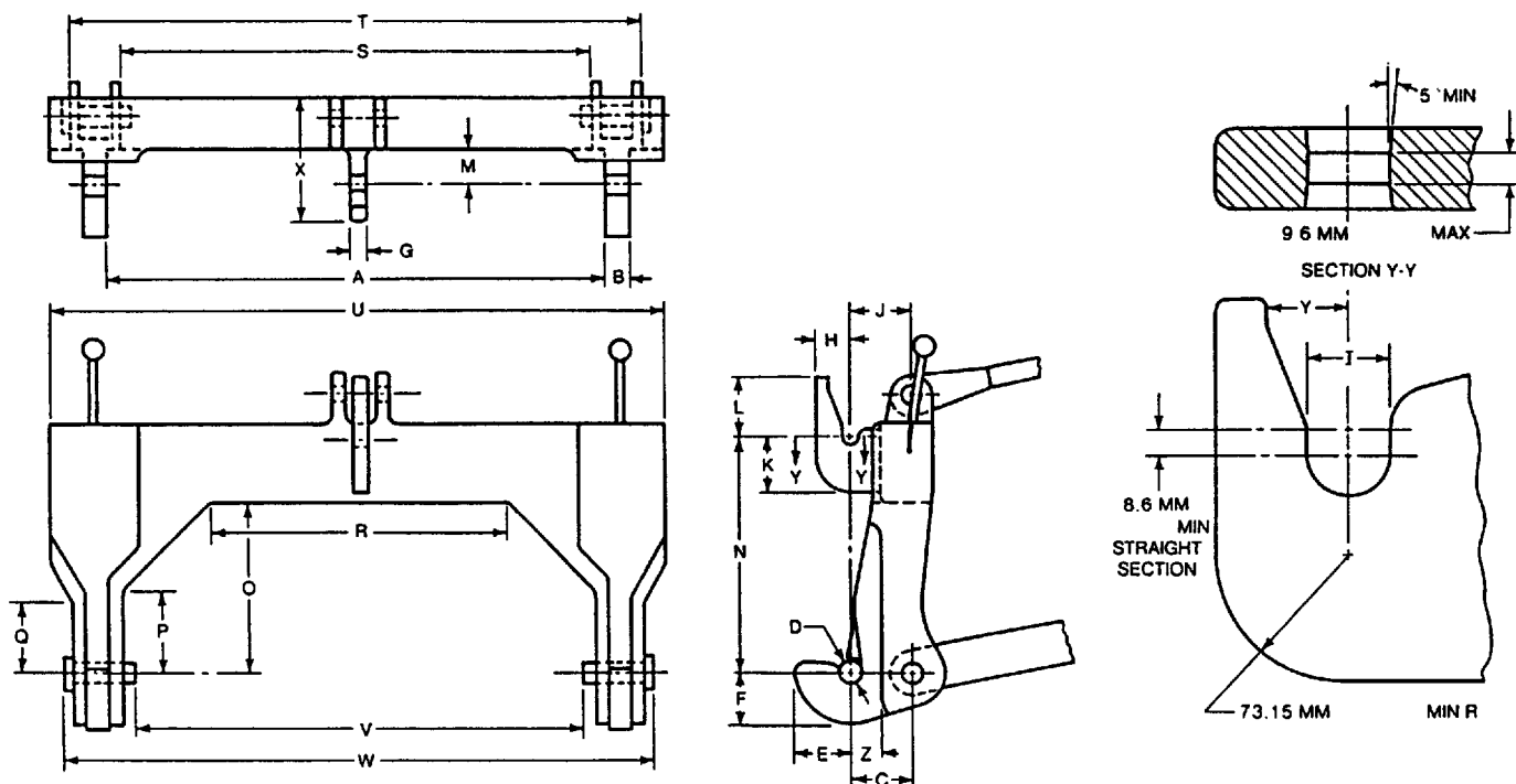
FIGURE 2—DIMENSIONS ASSOCIATED WITH QUICK-ATTACHING COUPLER (Letter designations A, B, C, etc., correspond to dimensions in Table 1)
