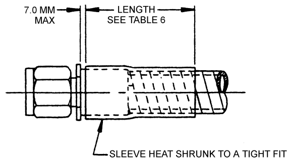
FIGURE 2 - SPIRAL ABRASION COVER /8/
