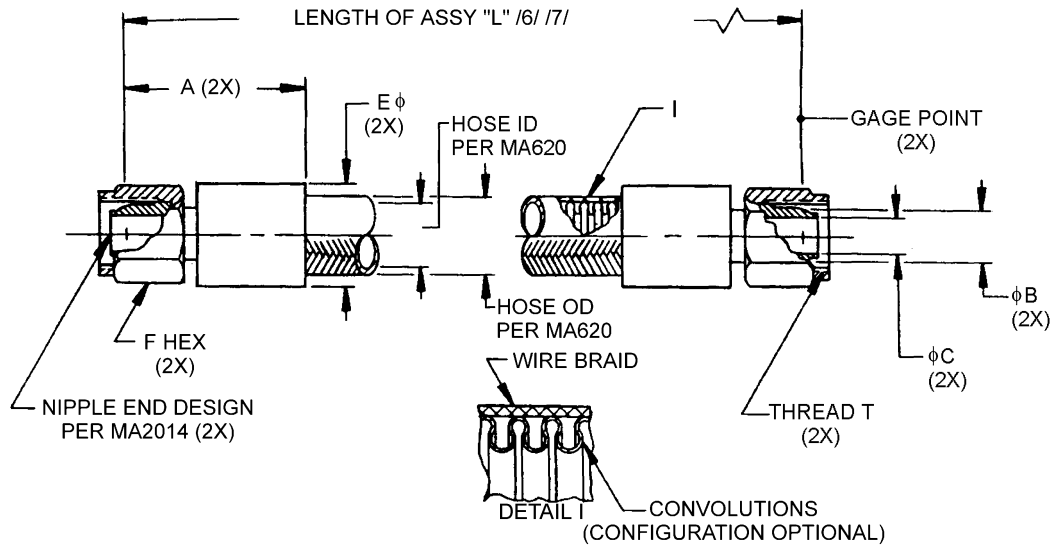
FIGURE 1 - HOSE ASSEMBLY
