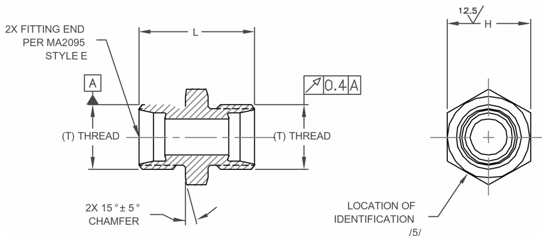
FIGURE 1 - UNION, NON-REDUCER
