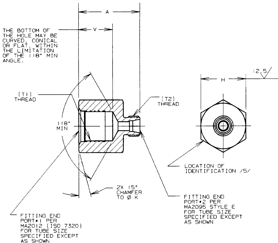
FIGURE 1 - BUSHING
