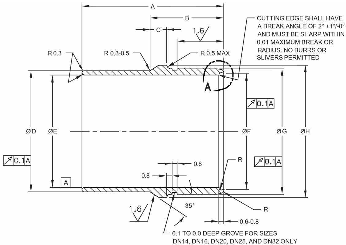
FIGURE 1 - SLEEVE DESIGN
