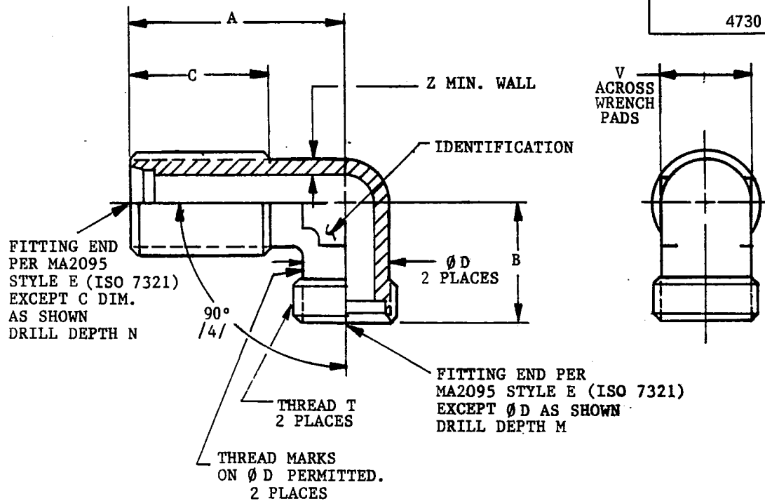
FIGURE 1 - FRONT AND SIDE VIEWS
