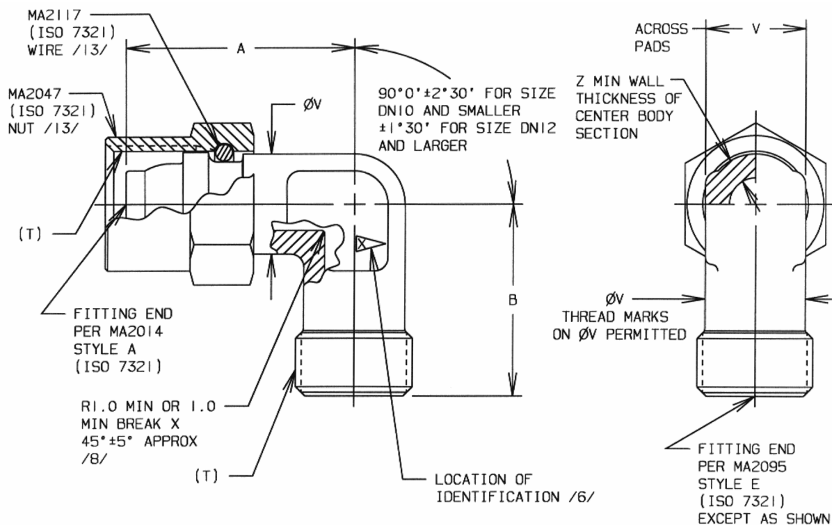
FIGURE 1 - ELBOW, 90°, FLARELESS
