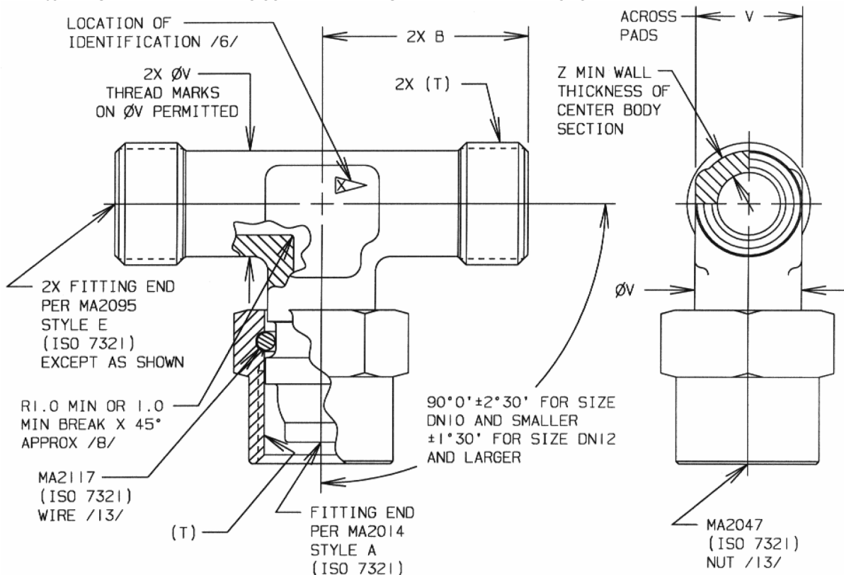
FIGURE 1 - ELBOW, 90°, FLARELESS
