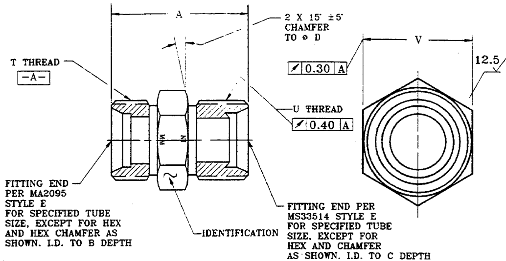
FIGURE 1 - FRONT AND SIZE VIEWS
