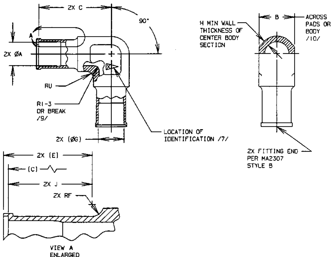
FIGURE 1 - FITTING, ELBOW, 90°
